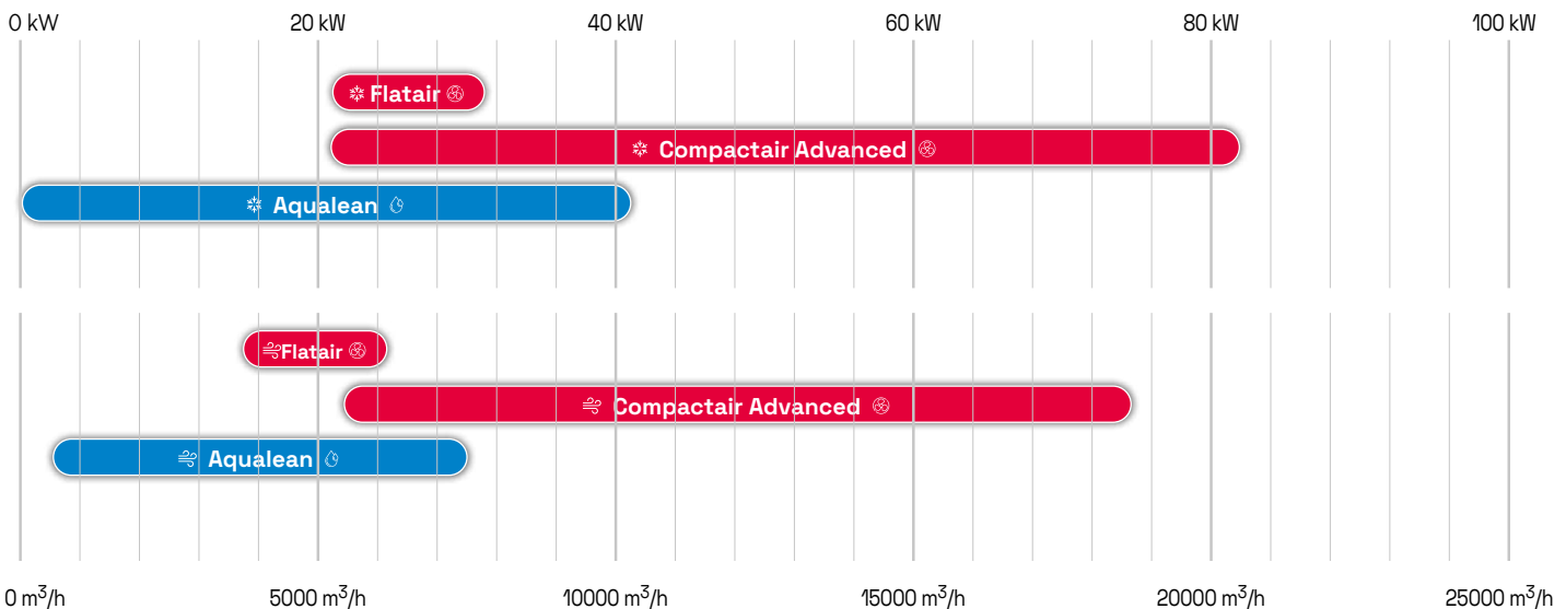
Cooling capacity
