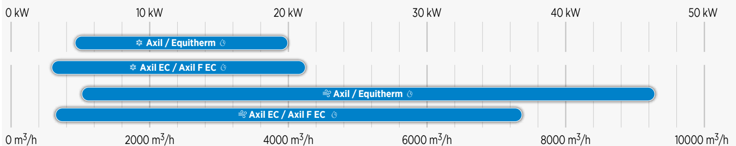
Cooling capacity
